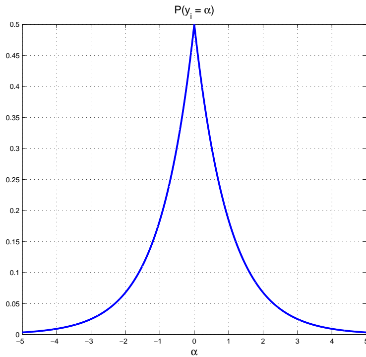
Figure A-1: Distribution of y_i for K = 2 , \tilde{\theta} \sim N(0, 1) and f_{i,j} \sim N(0, 1)
