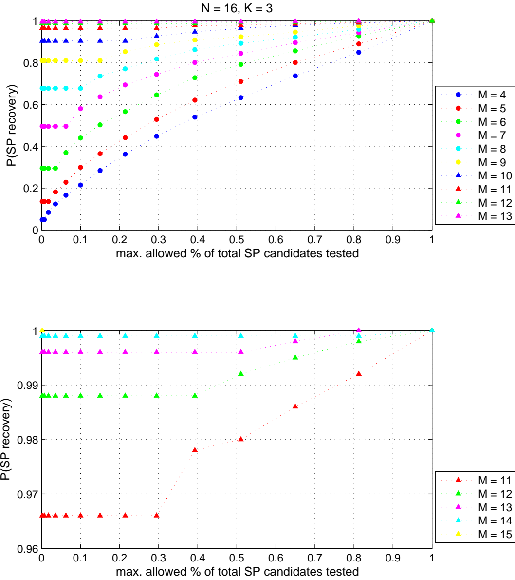
Figure 4-3: Probability of SP recovery by truncated BPOS for N = 16, K = 3 .
