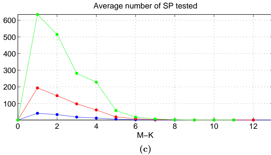
Figure 4-1: BPOS recovery performance. Note that the number of measurements is plotted as M - K .
