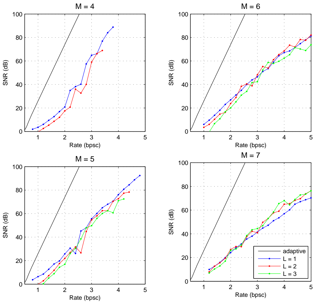
Figure 5-8: Nonadaptive D(R) for individual values of M \in [4 : 7] and different values of L .
