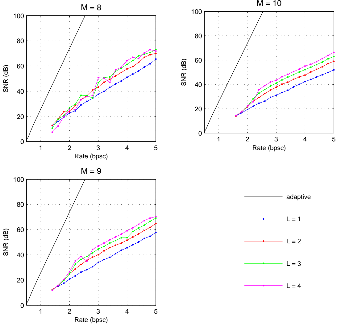
Figure 5-9: Nonadaptive D(R) for individual values of M \in [8 : 10] and different values of L .
