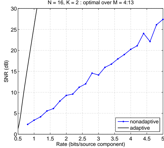
Figure 3-3: Comparison of adaptive and nonadaptive D(R) , where the nonadaptive decoder uses quantization-aware basis pursuit and the optimal value of M has been chosen for each rate.
